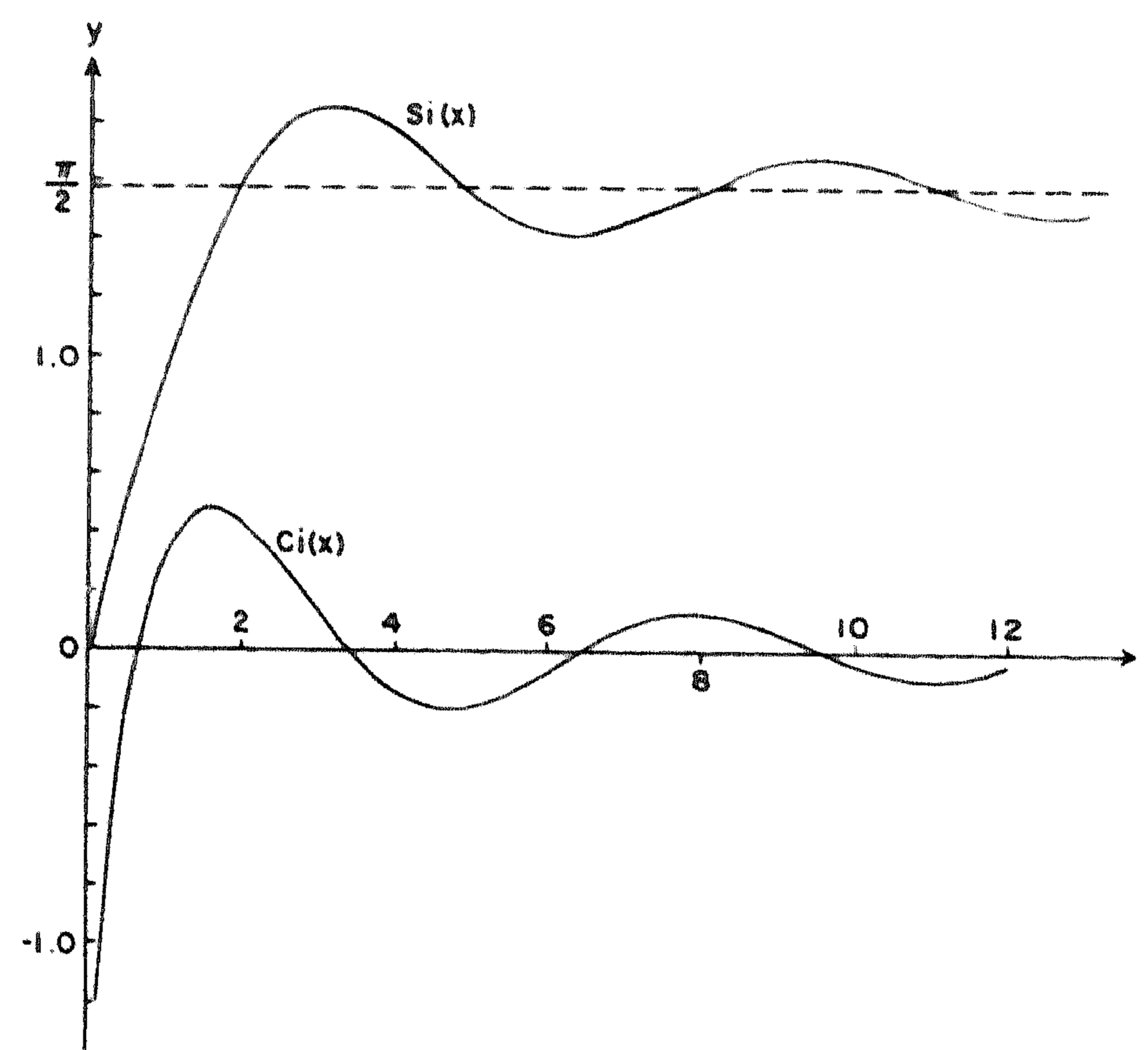
Figure 2. Graphs of Si(x) and Ci(x)
