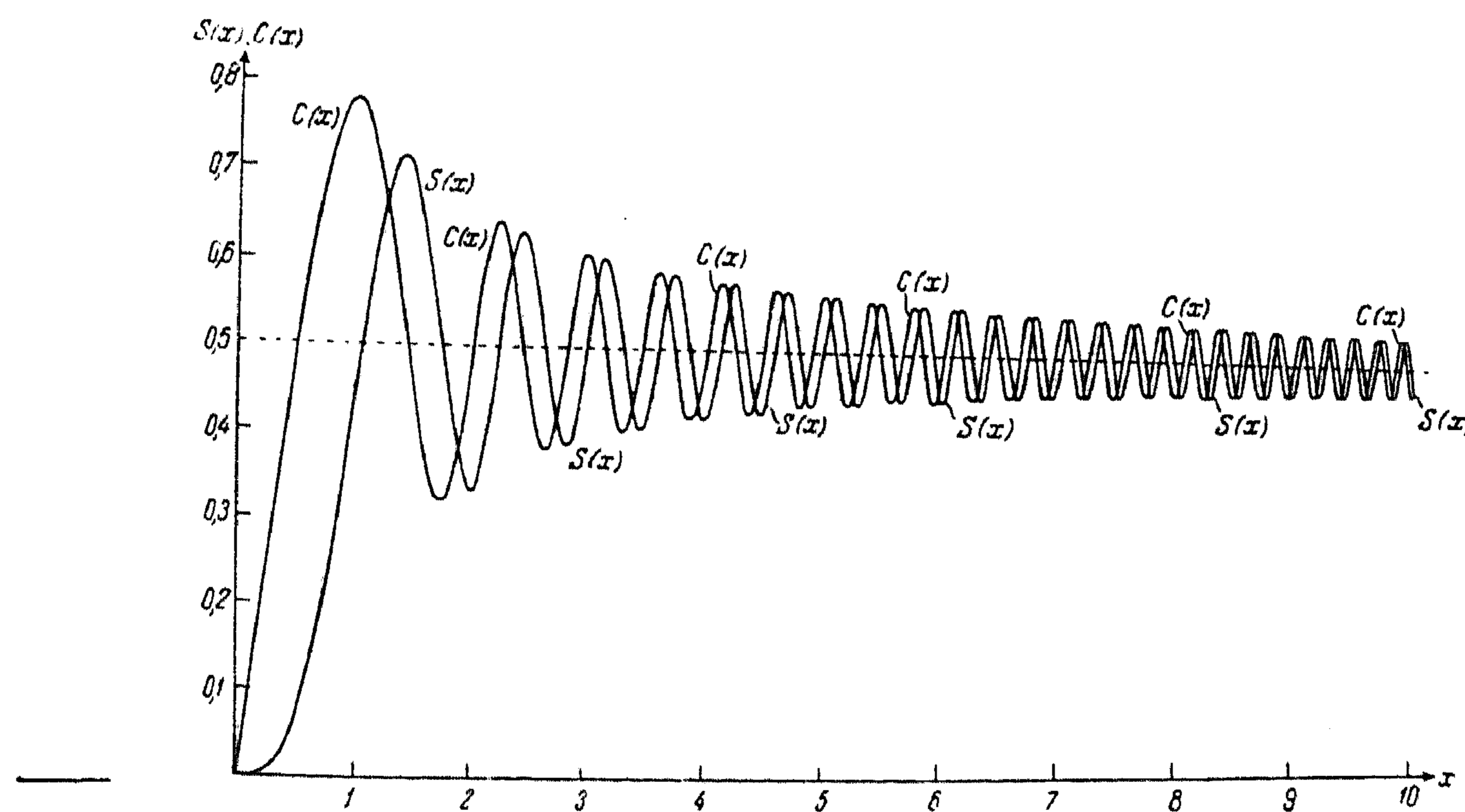
Figure 1. Graphs of S(x) and C(x) , x \geq 0 .
