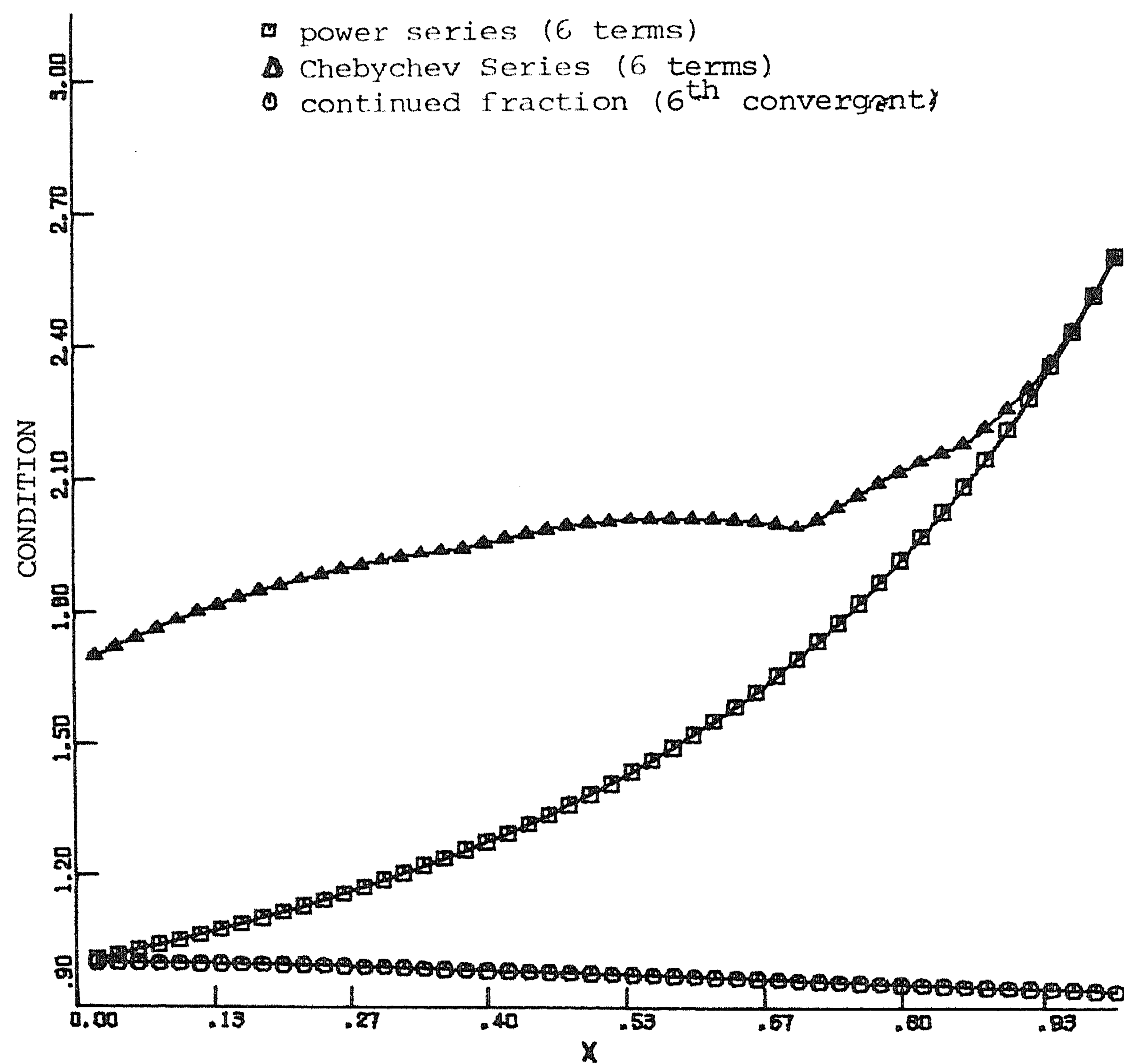
Figure 3. Condition of approximations for \ln(1+x)/x
