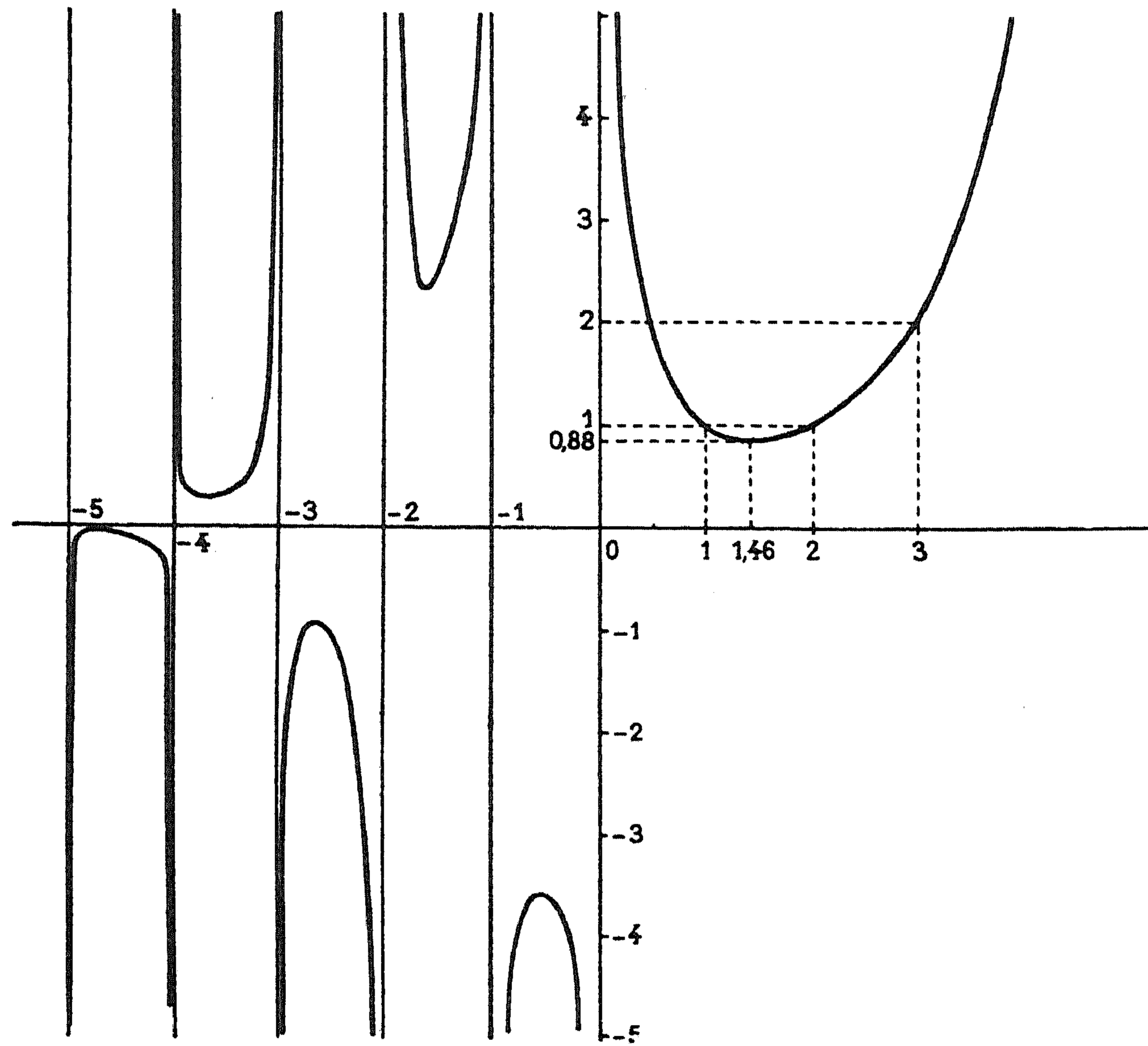
Figure 1. Graph of \Gamma(x) , x real
