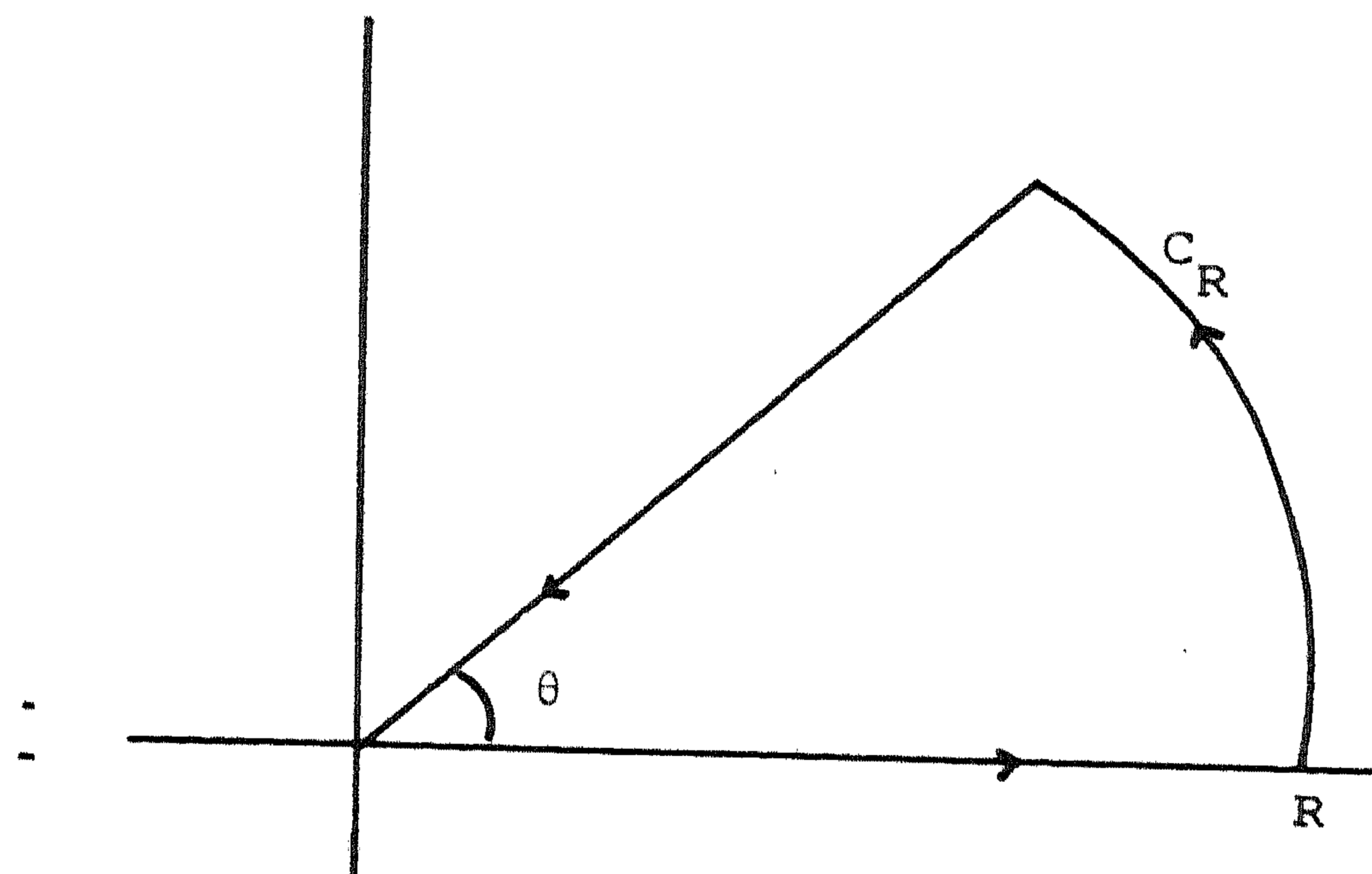
Figure 2. Contour of integration for (2.9).
