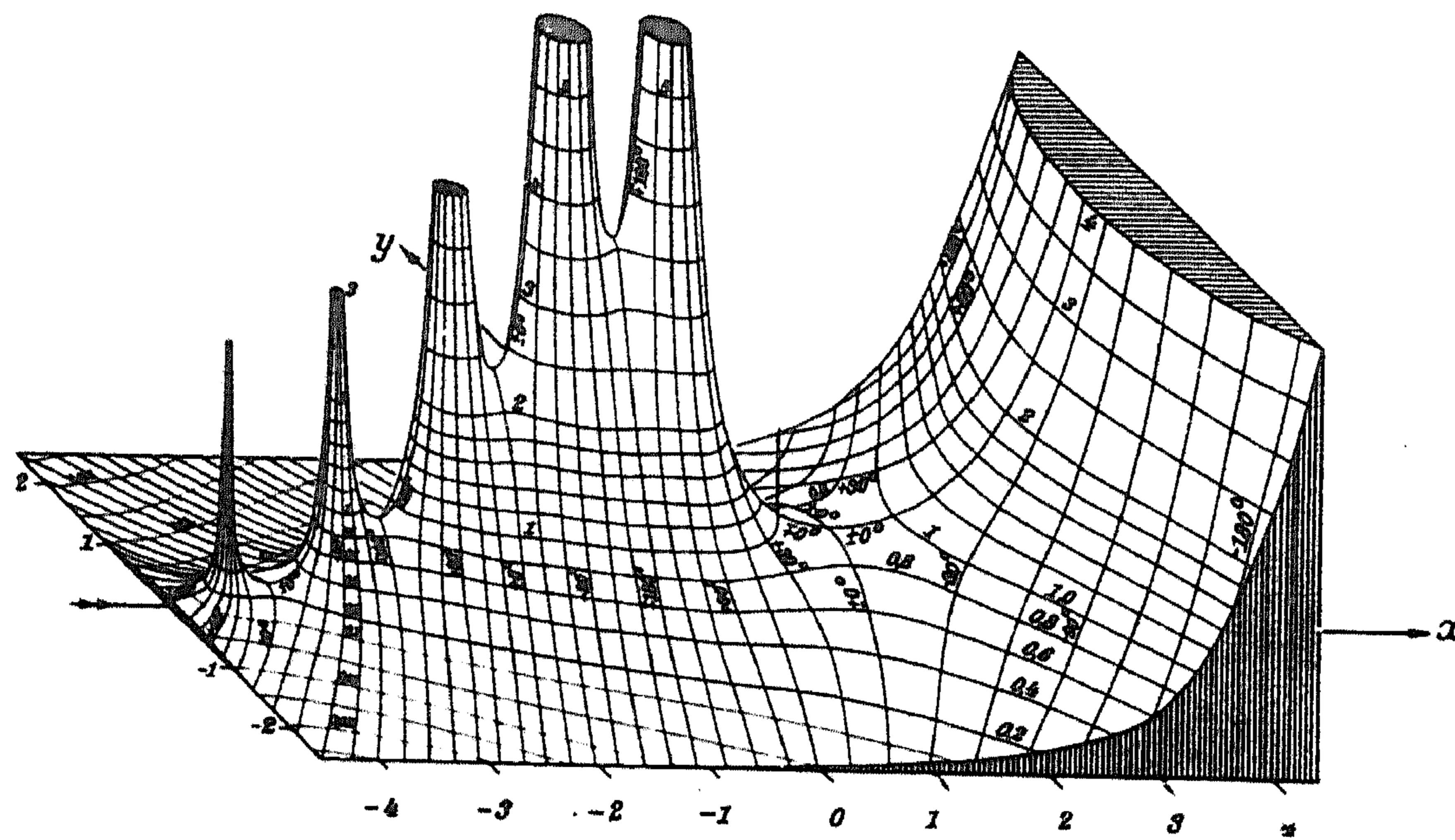
Figure 2. |\Gamma(z)| for complex z
