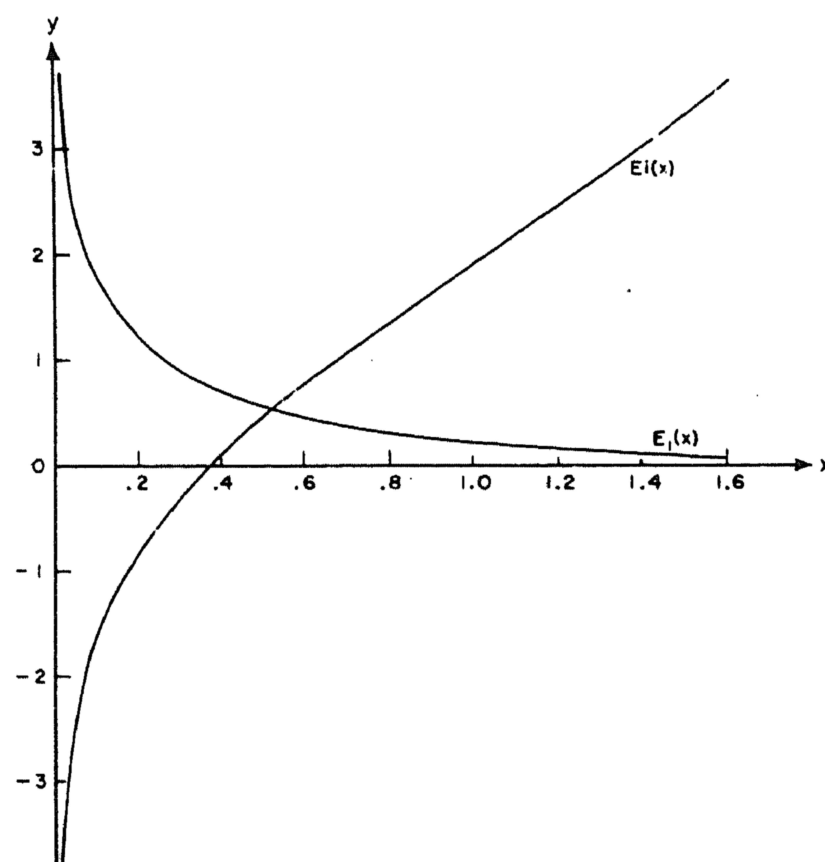
Figure 1. Graphs of \text{Ei}(x) and E_1(x)
